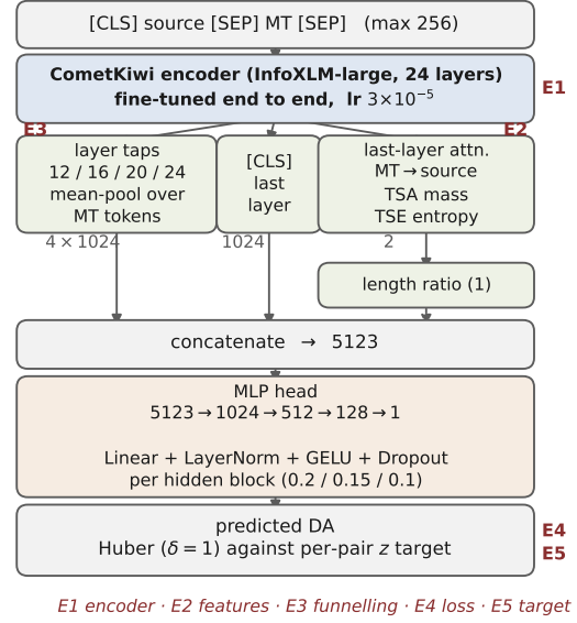
Figure 1: The regression head over a COMET encoder, and the five axes varied in Table 8. The encoder is fine-tuned with the head, not frozen. TSA is the MT-to-source attention mass and TSE its entropy.
