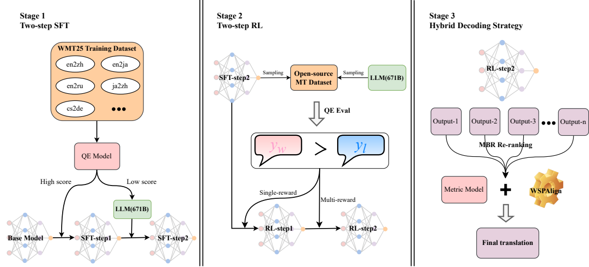
Figure 1: Overall pipeline of the Marco-MT-Algharb system. SFT Stage: Fine-tuning on QE-filtered and teacher-distilled data. RL Stage: Preference alignment via CPO and dynamic multi-reward optimization. Decoding Stage: Hybrid MBR re-ranking with a WSPAlign faithfulness score.
