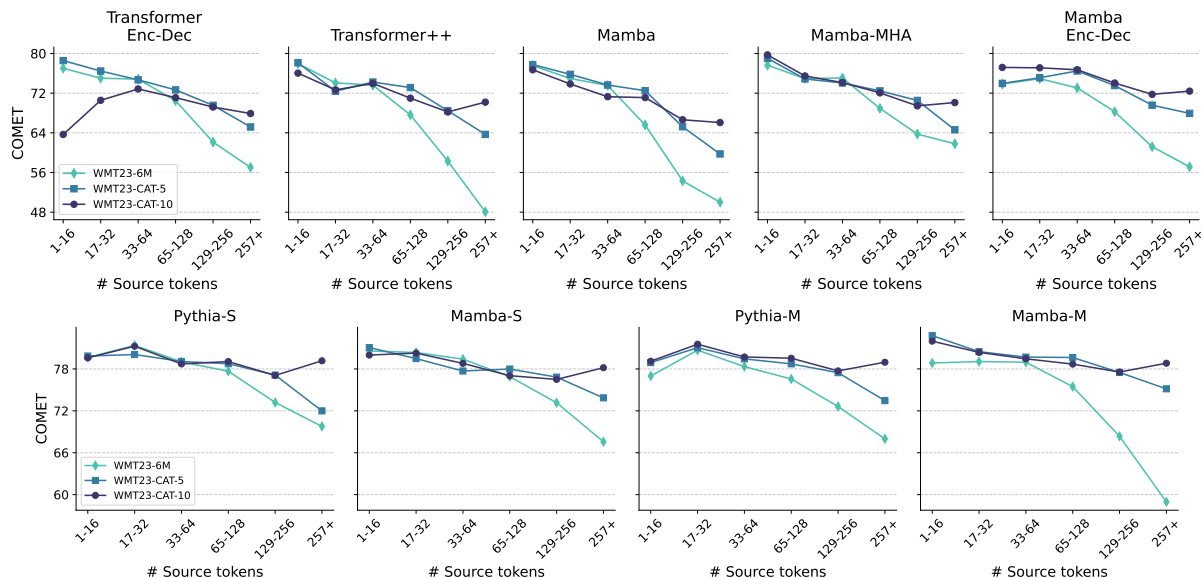
Figure 2: Sensitivity to input length, measured by the number of source tokens, on the WMT23 DE→EN dataset, for models trained from scratch (top) and finetuned from a pretrained checkpoint (bottom).
