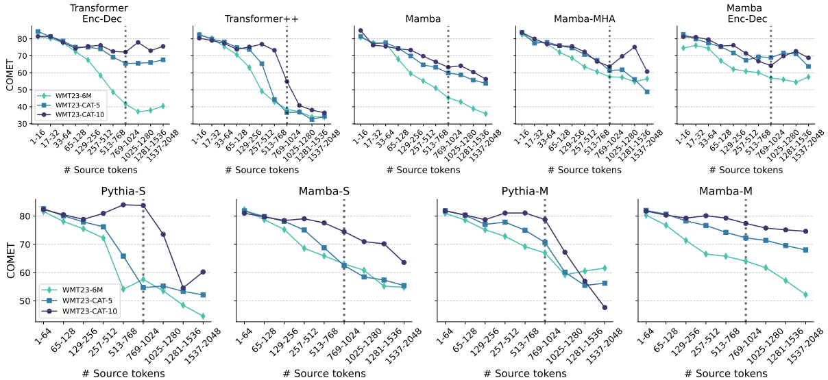
Figure 3: Sensitivity to input length, measured by the number of source tokens, on the Ted Talks DE→EN dataset, for models trained from scratch (top) and finetuned from a pretrained checkpoint (bottom). The dashed vertical line represents the bin containing the longest sentence in the training set.
